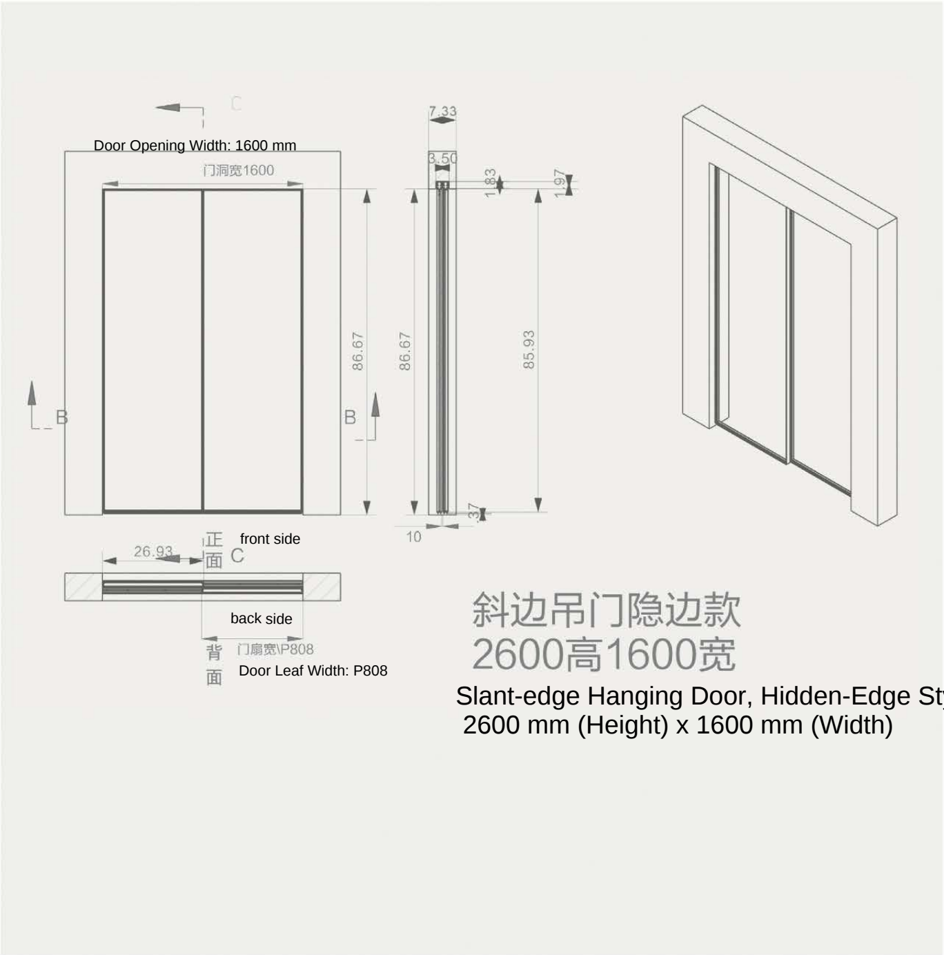
G3244 斜边吊门隐边款左右侧框加 G3244 Side Frame (Left & Right)
