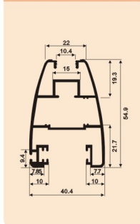
A1030 弧形光企 0.957kg/m
