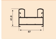
A1030 弧形光企 0.957kg/m
